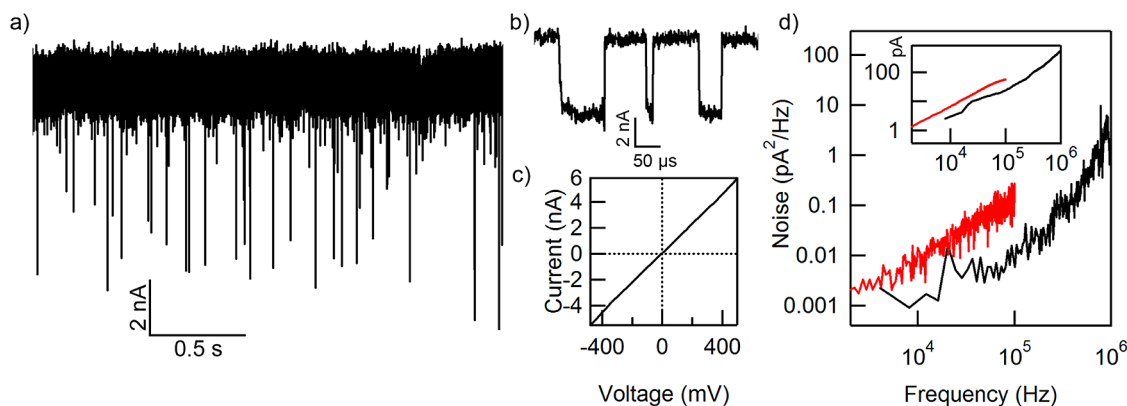
Figure 3. Characterization of noise in the \text{SiN}_x nanopores and the experimental setup using two amplifiers. (a) Raw current vs time trace for 50-mer ssDNA translocating through a 2-nm-diameter nanopore in a 5-nm-thick membrane with an applied bias of 1 V. The trace is digitally low-pass-filtered to B = 1 MHz. (b) Zoomed-in events from the trace in (a). Events have minimal attenuation and high signal-to-noise ratios. (c) Current vs voltage trace for a 2-nm-diameter nanopore in an 8-nm-thick membrane. The slope of this curve yields a conductance of 9.9 nS. (d) Input-referred noise power spectral density for a nanopore measured with an Axopatch 200B (red trace) and a nanopore measured with a Chimera VC100 (black trace). See Figure S4 in the Supporting Information for additional noise spectra. Inset: Calculated root-mean-square current noise for both amplifiers, as a function of signal bandwidth.
